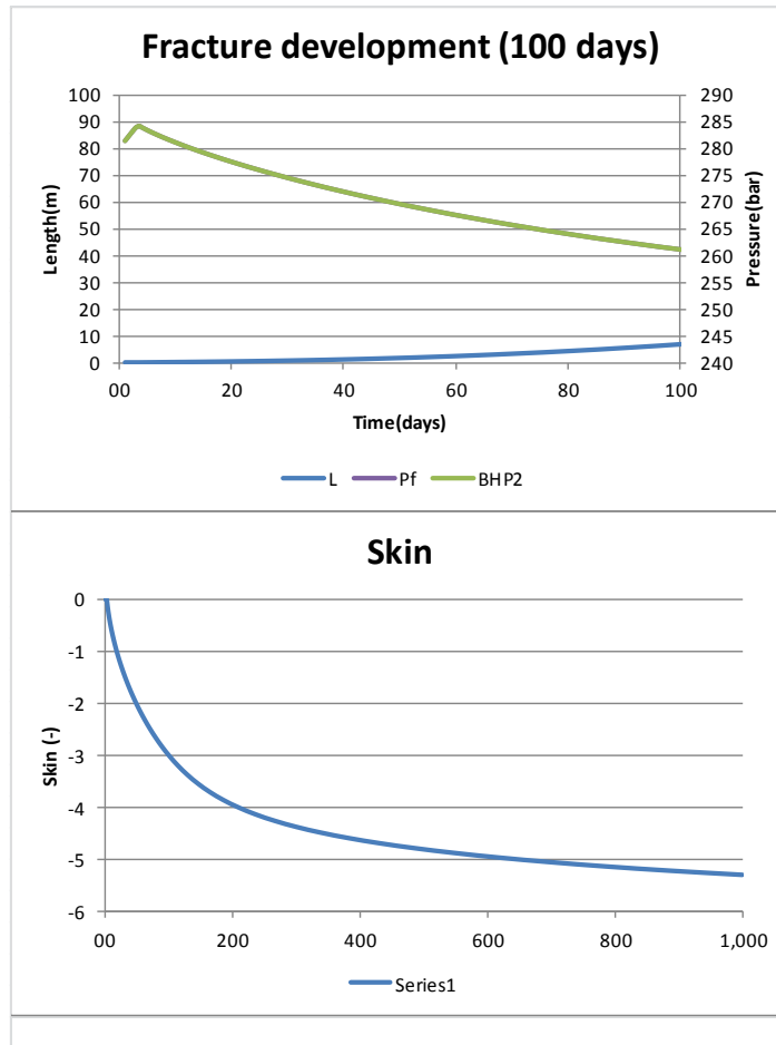
Figure 0.26 Visualization of the skin factor and fracture development over time
