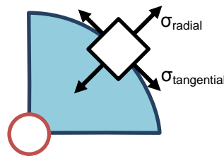
Figure 0.1 Plane view representation of the radial and tangential components of the thermal stress in a horizontal plane. Injection well in red, cold front in blue.
