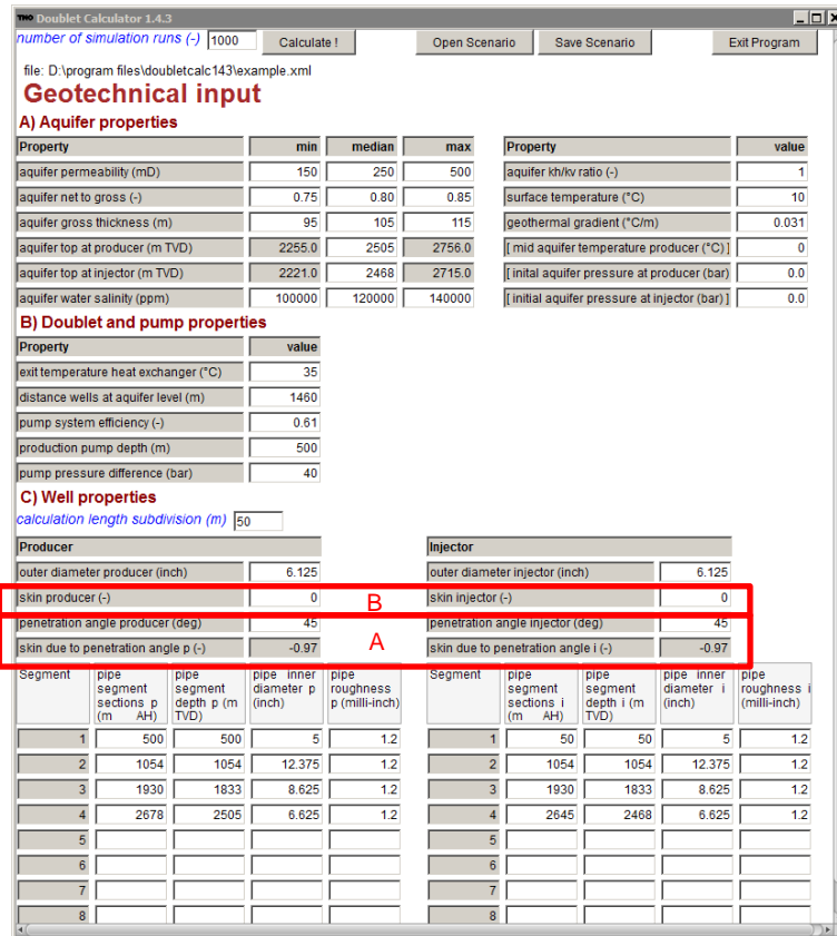
Figure 3.9 DoubletCalc input screen showing well inclination and automatically calculated penetration angle skin (A). Additionally, a 'skin producer' and / or 'skin injector' can be specified manually (B).
