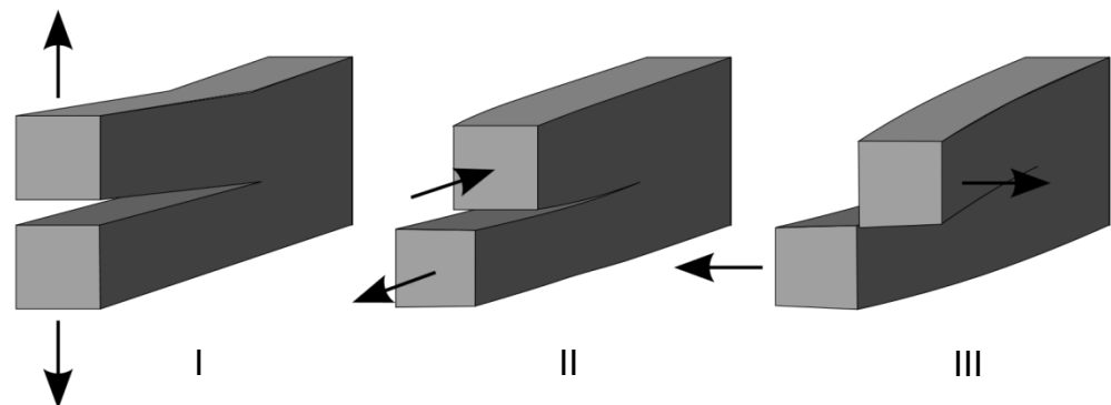
Figure 3.2 Three modes of fracture mechanics (I: opening, II: in-plane shear and III: out-of-plane shear). Source: wikimedia.
