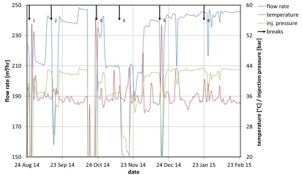
Figure 4.3 Complete production data D1 doublet (daily average) showing flow rate, injection temperature and injection pressure.
