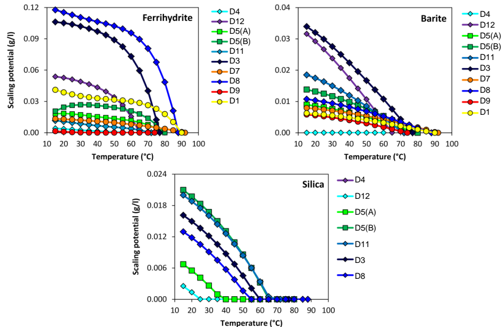
Figure 5.15.4 Scaling potential of ferrihydrite, barite and silica (in g/l) with cooling as predicted for various geothermal doublets of the Netherlands.
