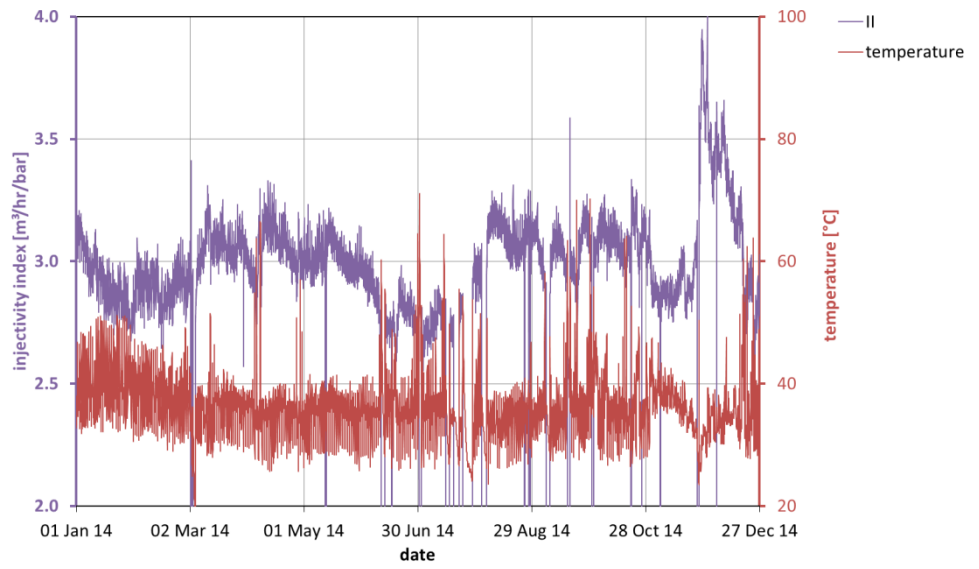
Figure 0.39 Injectivity index and temperature of the D3 doublet.
