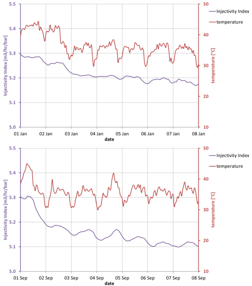
Figure 0.36 Production data D1 doublet for the same two weeks as Figure 0.32, showing injectivity index and temperature
