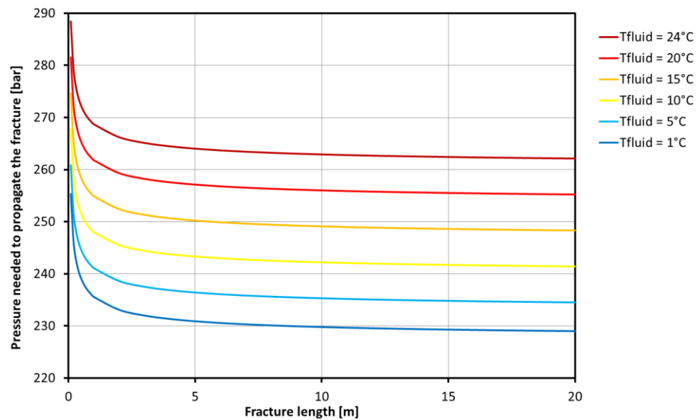
Figure 0.12 Injection pressure required to propagate the initial 9 cm long fracture for different fluid temperatures (coefficient of thermal expansion = 10 \cdot 10^{-6} [1/C]).
