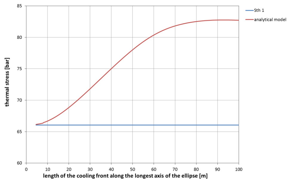
Figure 0.15 Thermal stress calculated using the analytical model eq. 3.
