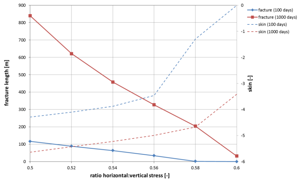
Figure 3.7 Fracture and skin development for a 'typical' doublet using varying horizontal : vertical stress ratios.
