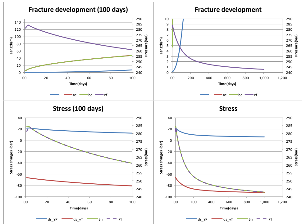
Figure 0.24 Input tab sheet graphics showing the fracture and stress development in the geothermal doublet over time. Upper panels: L: fracture length; ac, bc: long and short axis of the ellipsoid of the cold front; Pf: pressure in the fracture. Lower panels: ds_yP: change of the initial stress perpendicular to the fracture due to poro-elastic effects (positive); ds_yT: change of the initial stress perpendicular to the fracture due to thermal-elastic effects (negative); Sh: current stress at the tip of the fracture; Pf: pressure in the fracture, which is equal to the initial stress from the moment the fracture starts to propagate.
