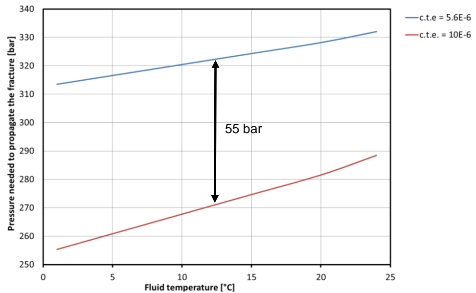
Figure 0.13 Pressure required to propagate the initial fracture as function of the fluid temperature, for two values of the coefficient of thermal expansion (c.f. Figure 0.11, Figure 0.12).
