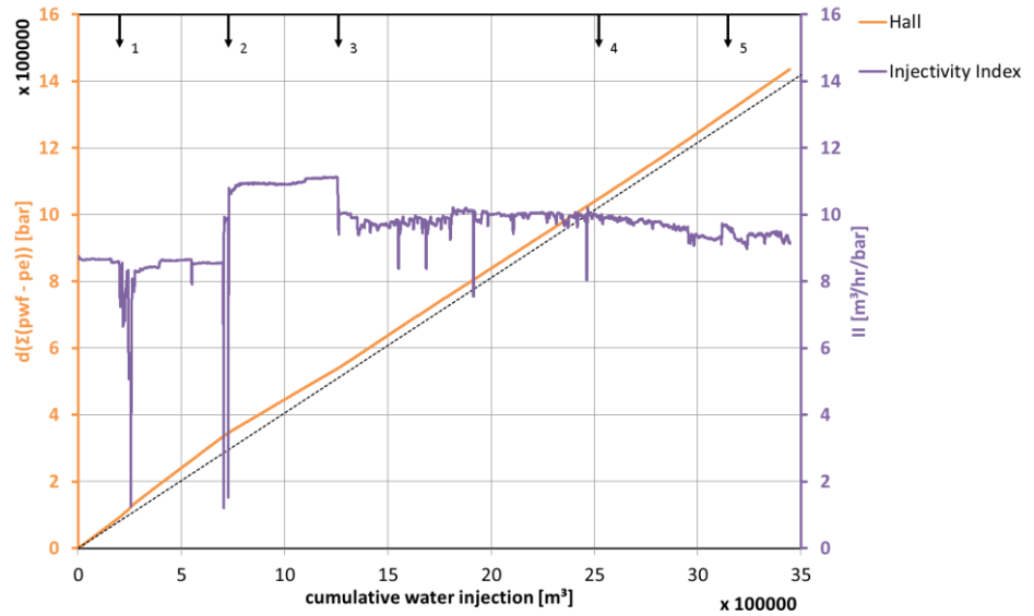
Figure 0.44 Hall plot and injectivity index of the D4 doublet. Arrows indicate changes in injectivity index.
