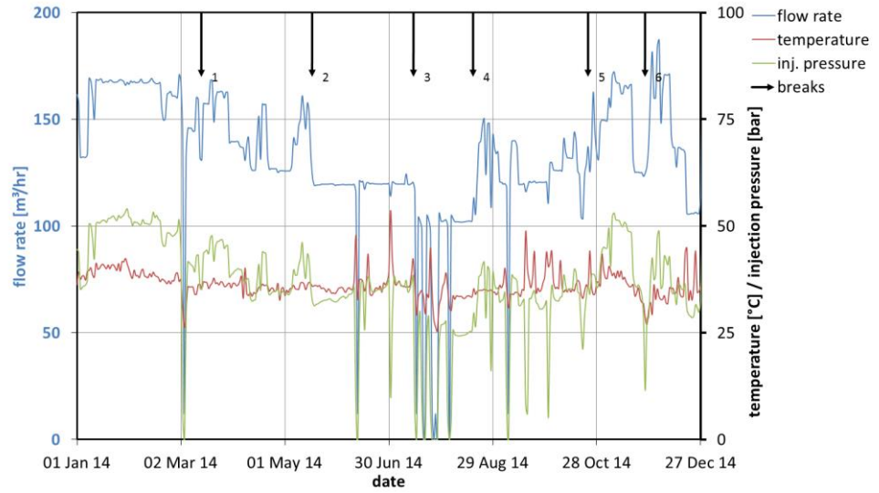
Figure 0.37 Complete production data D3 doublet (daily average) showing flow rate, injection temperature and injection pressure.
