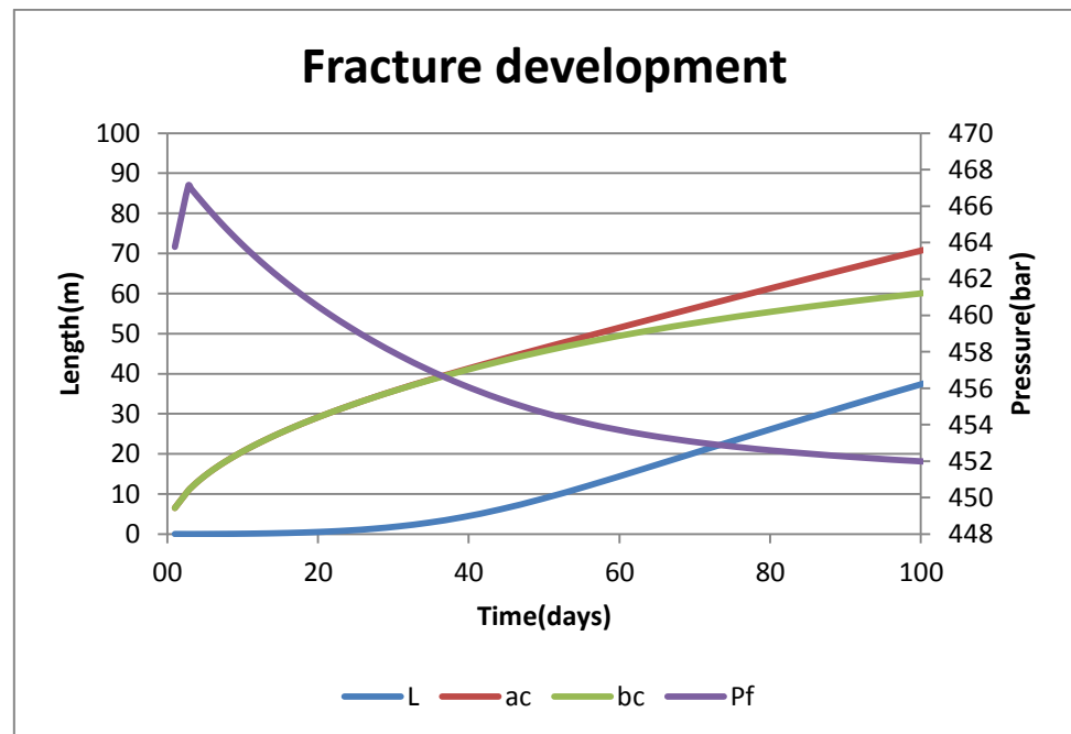
Figure 0.6 Propagation of the fracture (L), long axis of the heat front ellipsoid (ac), short axis of the heat front ellipsoid (bc) and pressure in the fracture (Pf).
