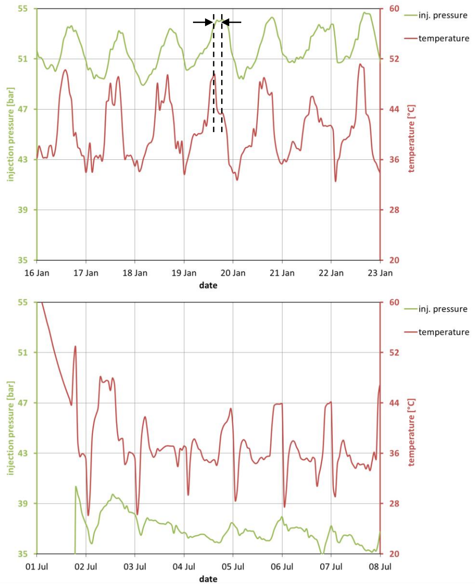
Figure 0.41 Production data D3 doublet for the same two weeks as Figure 0.40, showing injection temperature and pressure. Arrows indicate the time shift between injection temperature reduction and injection pressure reduction.
