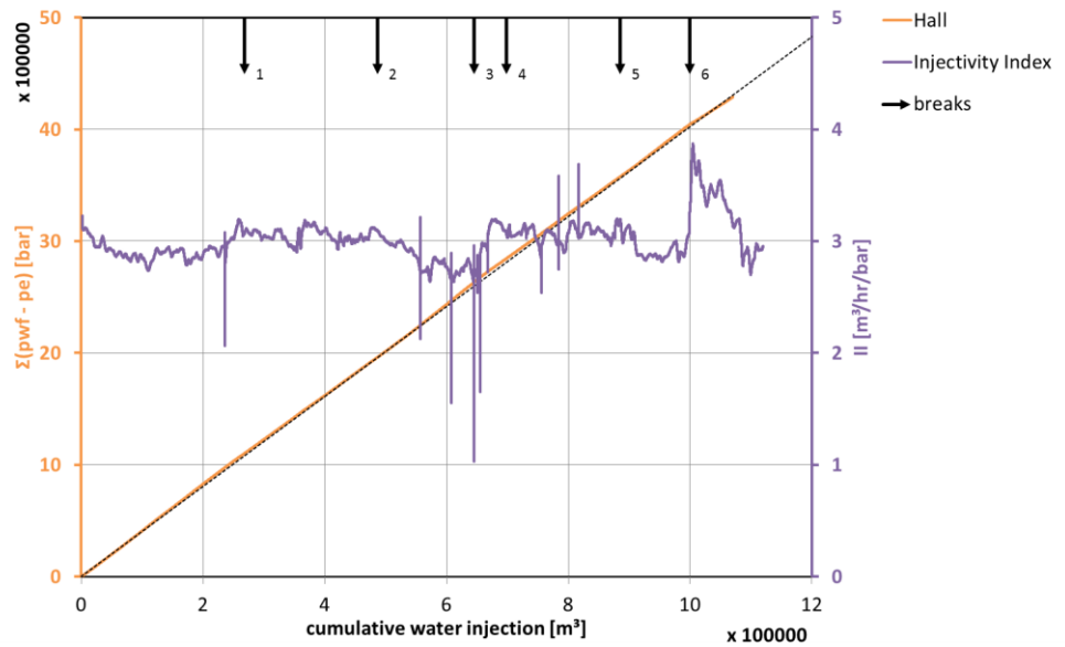
Figure 0.38 Hall plot and injectivity index of the D3 doublet.
