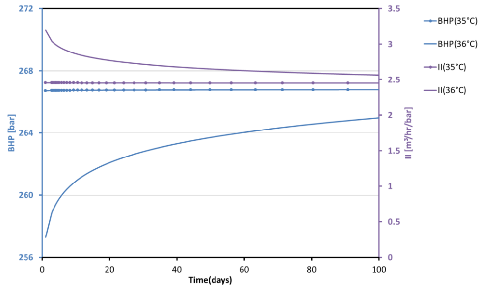
Figure 0.21 Development of BHP and injectivity index with constant injection rate of 4800 m 3 /day with constant injection temperature of 35°C, and including time dependent heating (indicated by calculated temperature of 36°C).
