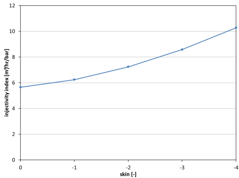
Figure 3.8 Theoretical relation between negative skin (for instance, fracture induced) and injectivity index for a 'typical' doublet. The increase in injectivity index is in the order of tens of percent for a (very high) skin of -4.
