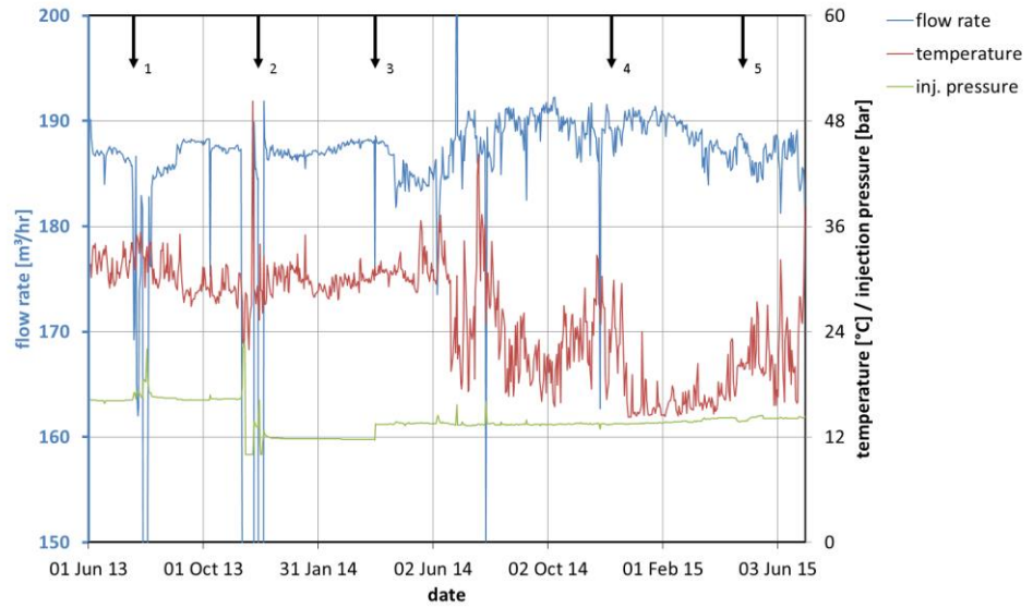
Figure 0.43 Complete production data D4 doublet (daily average), showing flow rate, injection temperature and injection pressure.
