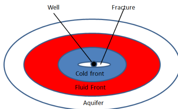
Figure 3.4 Elliptical shape of the cold and fluid fronts around the injection well (top view).
