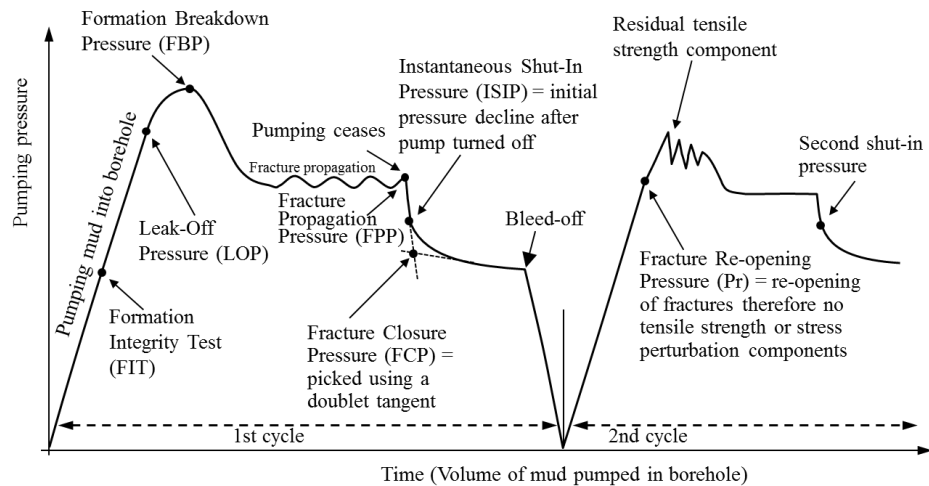
Figure 0.27 Example of an 'ideal' extended leak-off test (redrawn after Lin et al. 2008).
