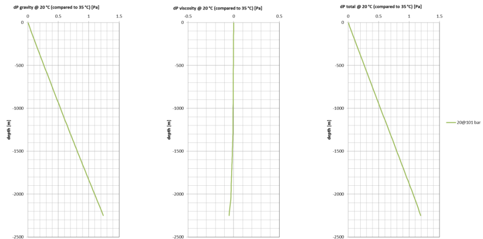
Figure 2.4 Increased pressure due to density effect (left), viscosity effect (middle) and combined effects (right) for increased cooling to 20°C @101 bar pump pressure difference.
