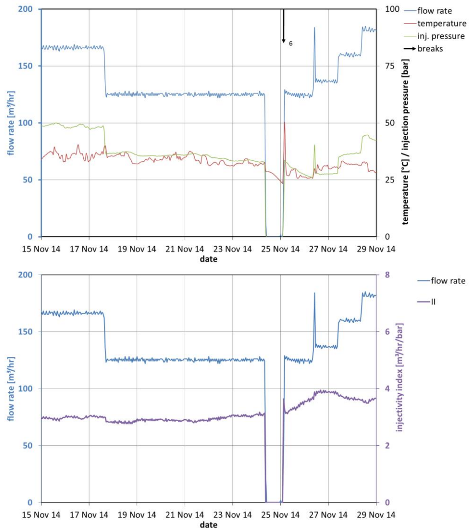
Figure 4.9 D3 doublet production data for two weeks in November showing flow rate, temperature, injection pressure and injectivity index.
