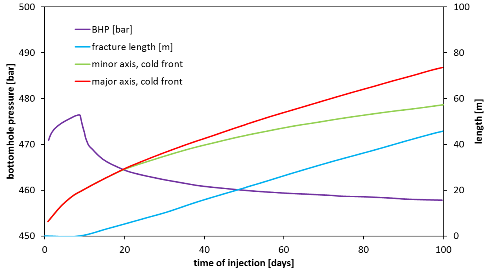
Figure 0.7 Simulation output after Koning
