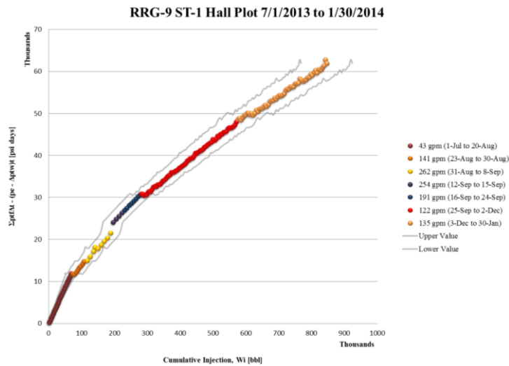
Figure 4.2 Field example of a hall plot analysis on an injector well in the Raft River geothermal field (Bradford et al., 2014). 'Cooler' colours represent cold water injection.
