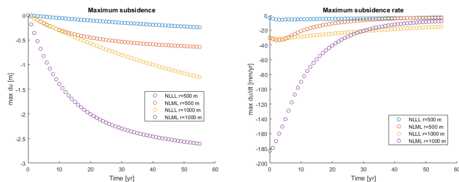
Figure 8-4: Total subsidence and subsidence rate at the centre of the subsidence bowl, for the NLML and NLLL cases. After 5 years, the cavern pressure is switched from halmostatic to 90% of the in-situ stress.
