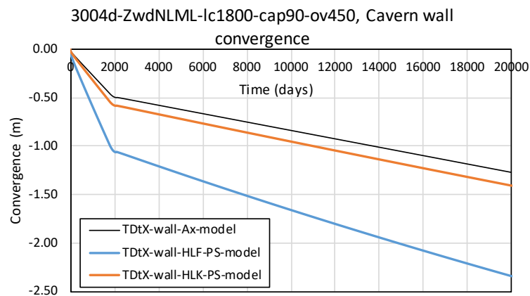
Figure 7-6: Comparison of cavern wall convergence (horizontal displacement) from the axis-symmetric model (black line, TDtX-wall-Ax-model), the plane strain model with the HL-F cavern (blue line, TDtX-wall-HLF-PS-model) and the plane strain model with the HL-K cavern (TDtX-wall-HLK-PS-model). The medium linear creep case. The agreement is good between the caverns of similar radius (i.e. the axisymmetric model and the plane strain model with HL-K cavern).
