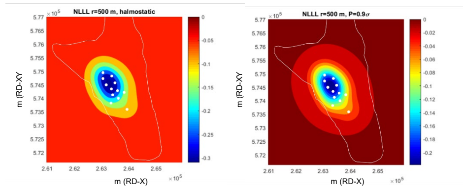
Figure 9-1: Contours of total subsidence [in m] during 50 years of shut-in, for the 500-m salt dome with the NLLS creep law, for the complete cavern field. Left: for hallowstatic cavern pressure. Right: cavern pressure increased to 90% of the virgin stress magnitude. The white dots show cavern locations. The white line represents the outline of the Winschoten dome at -1.500m
