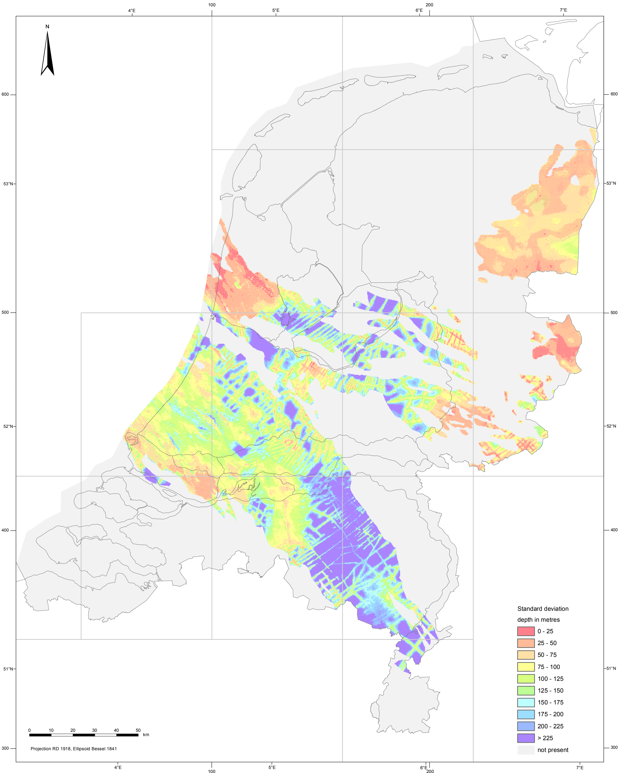
Uncertainty (standard deviation) of the depth of the base of the Altena Group (AT)
