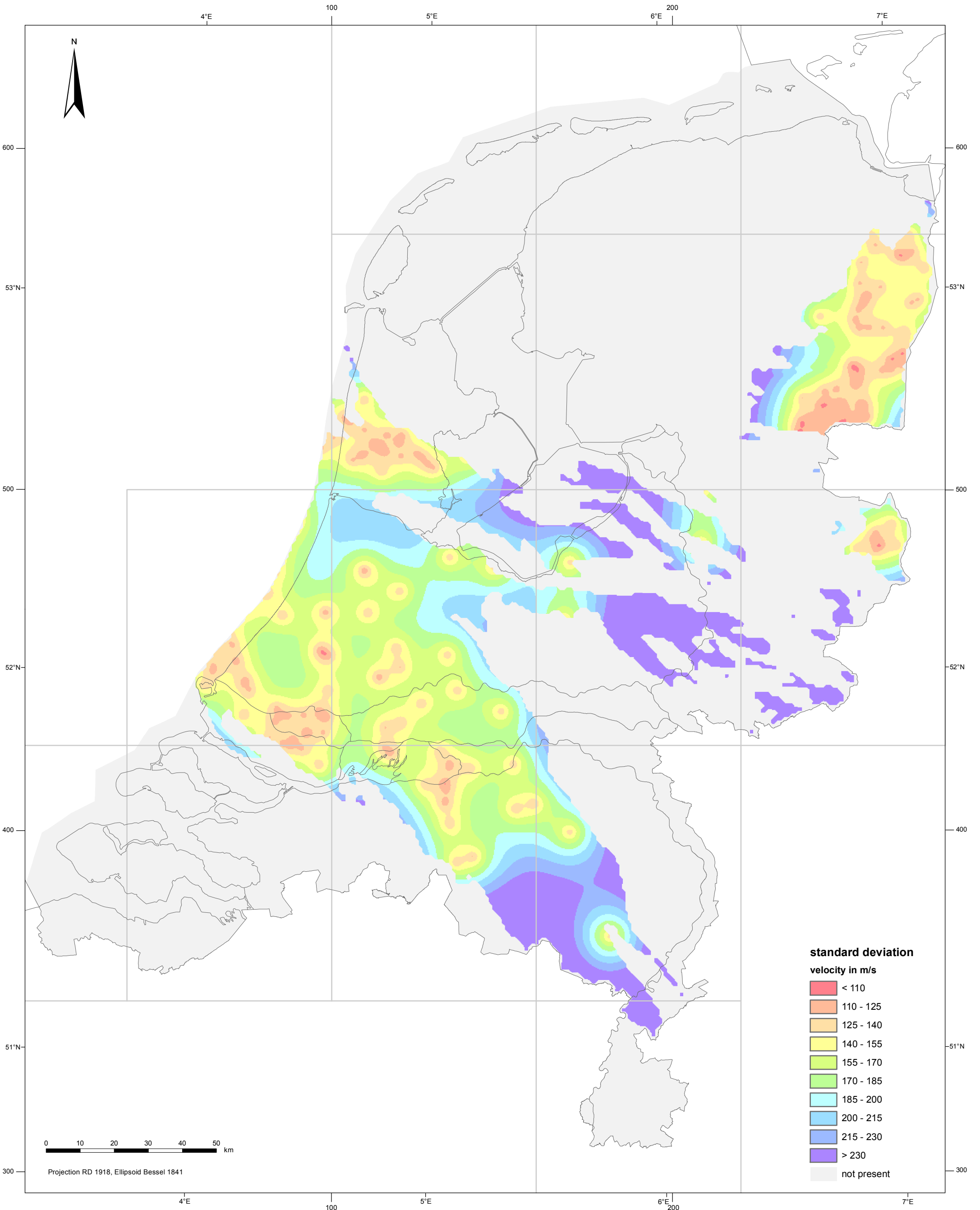
Uncertainty (standard deviation) of the velocity ( V_0 ) of the Altena Group (AT)
