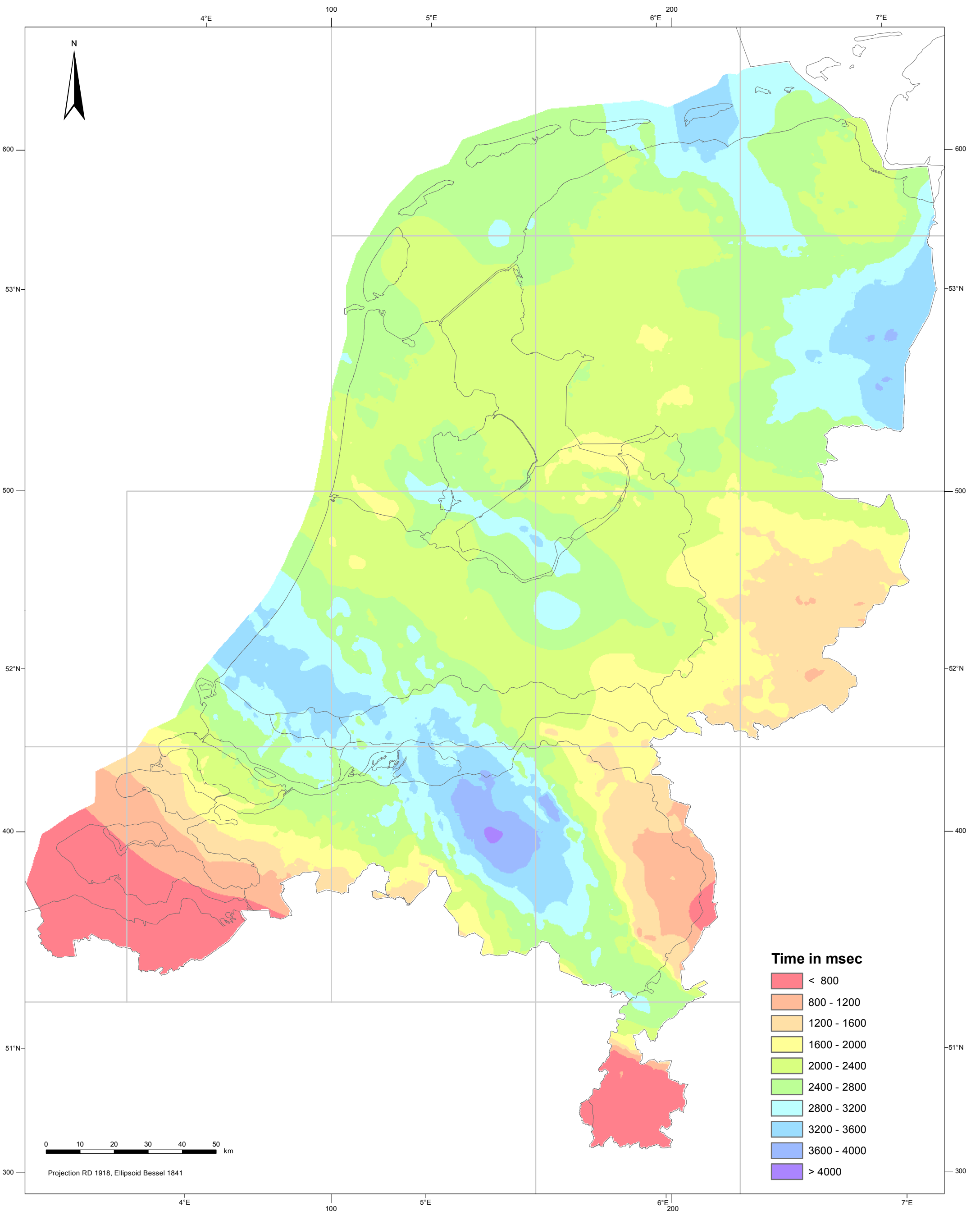
Two Way Time (TWT) of the base of the Caumer, Dinkel and Hunze subgroups (DCC)
