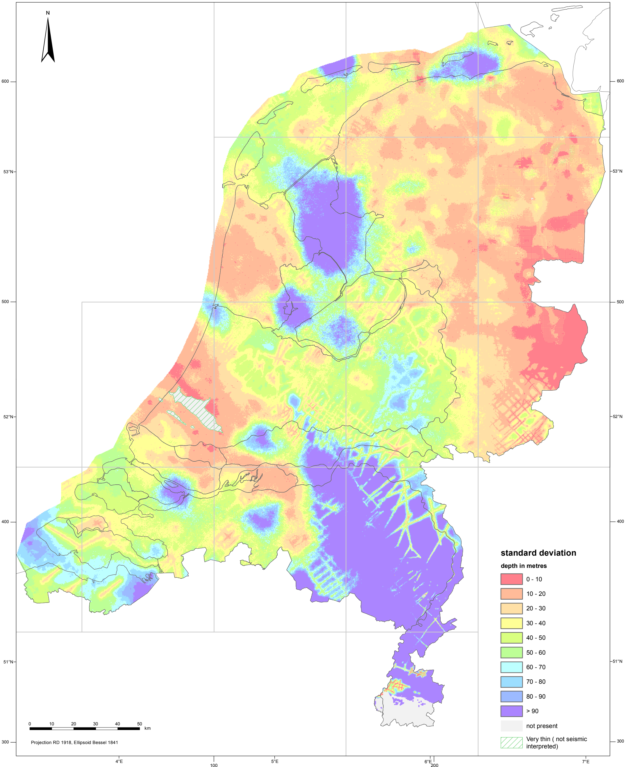
Uncertainty (standard deviation) of the depth of the base of the North Sea Supergroup (N)
