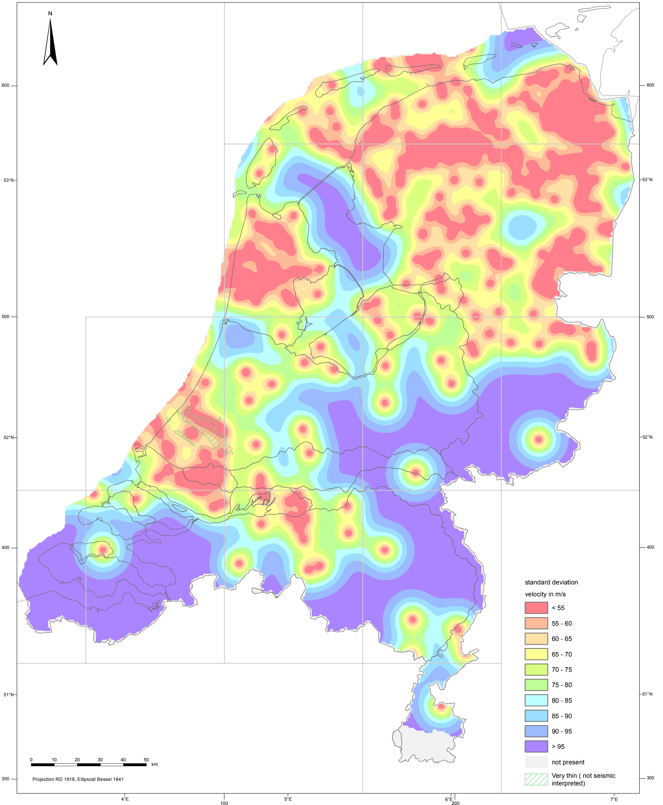
Uncertainty (standard deviation) of the velocity ( V_0 ) of the North Sea Supergroup (N)
