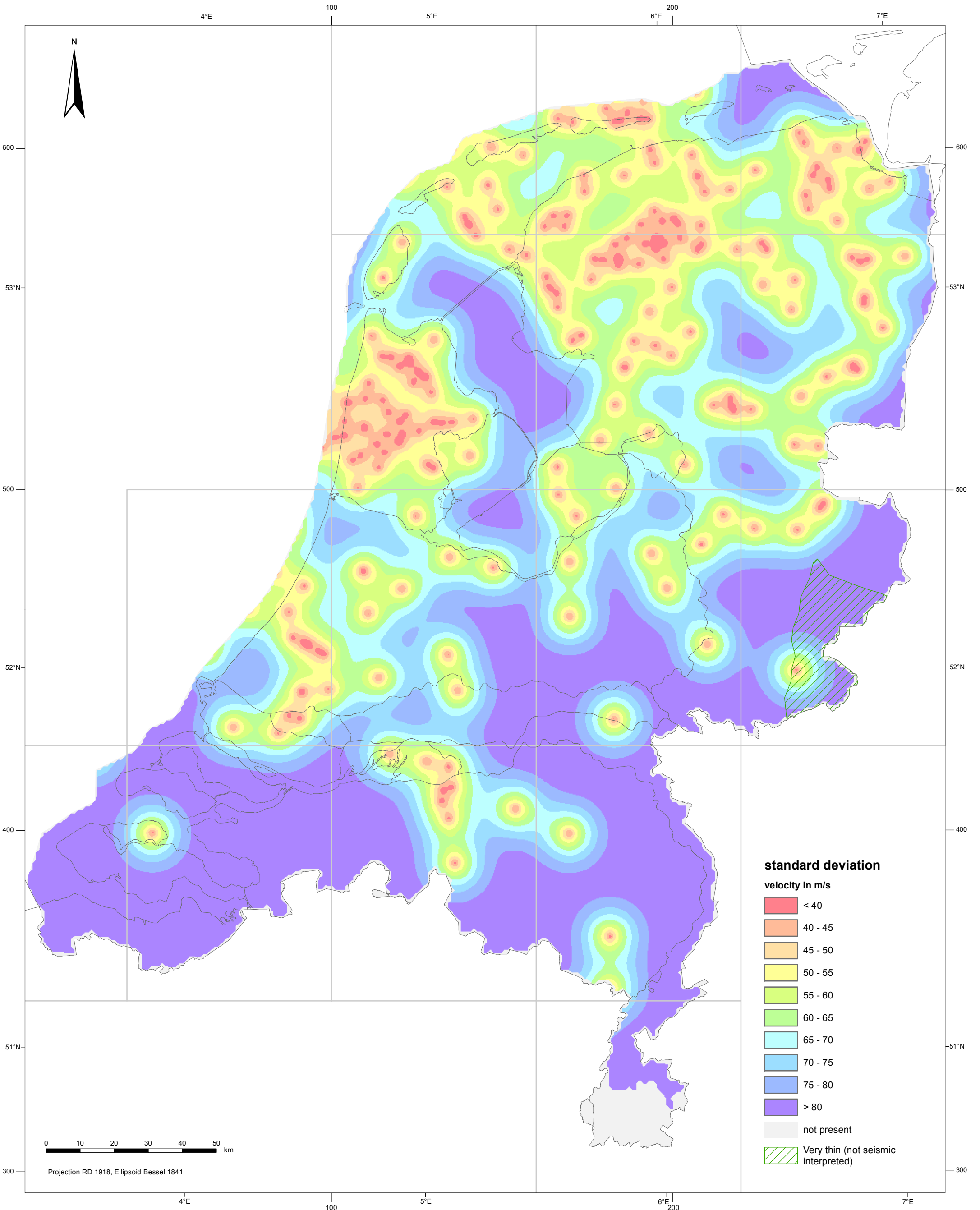
Uncertainty (standard deviation) of the velocity ( V_0 ) of the Upper North Sea Group (NU)
