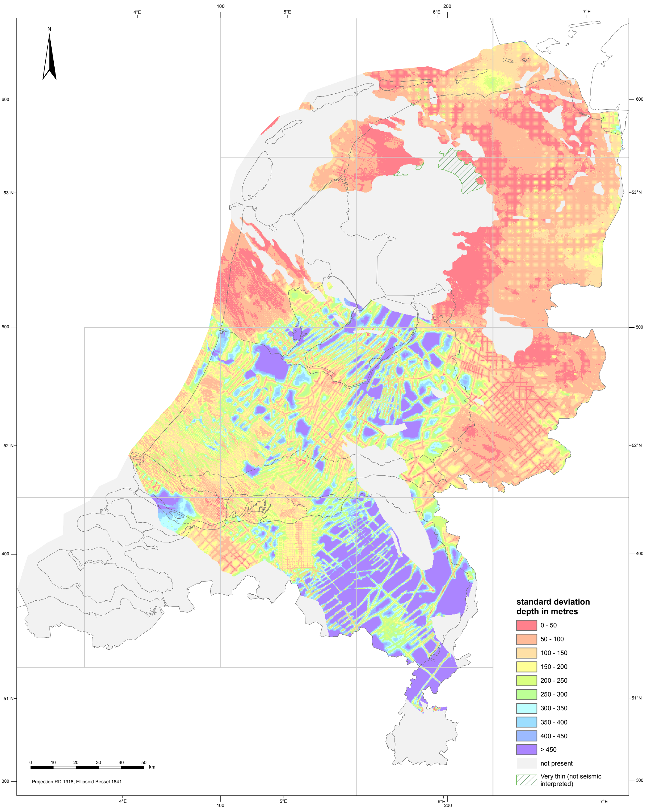
Uncertainty (standard deviation) of the base of the Lower Germanic Trias Group (RB)
