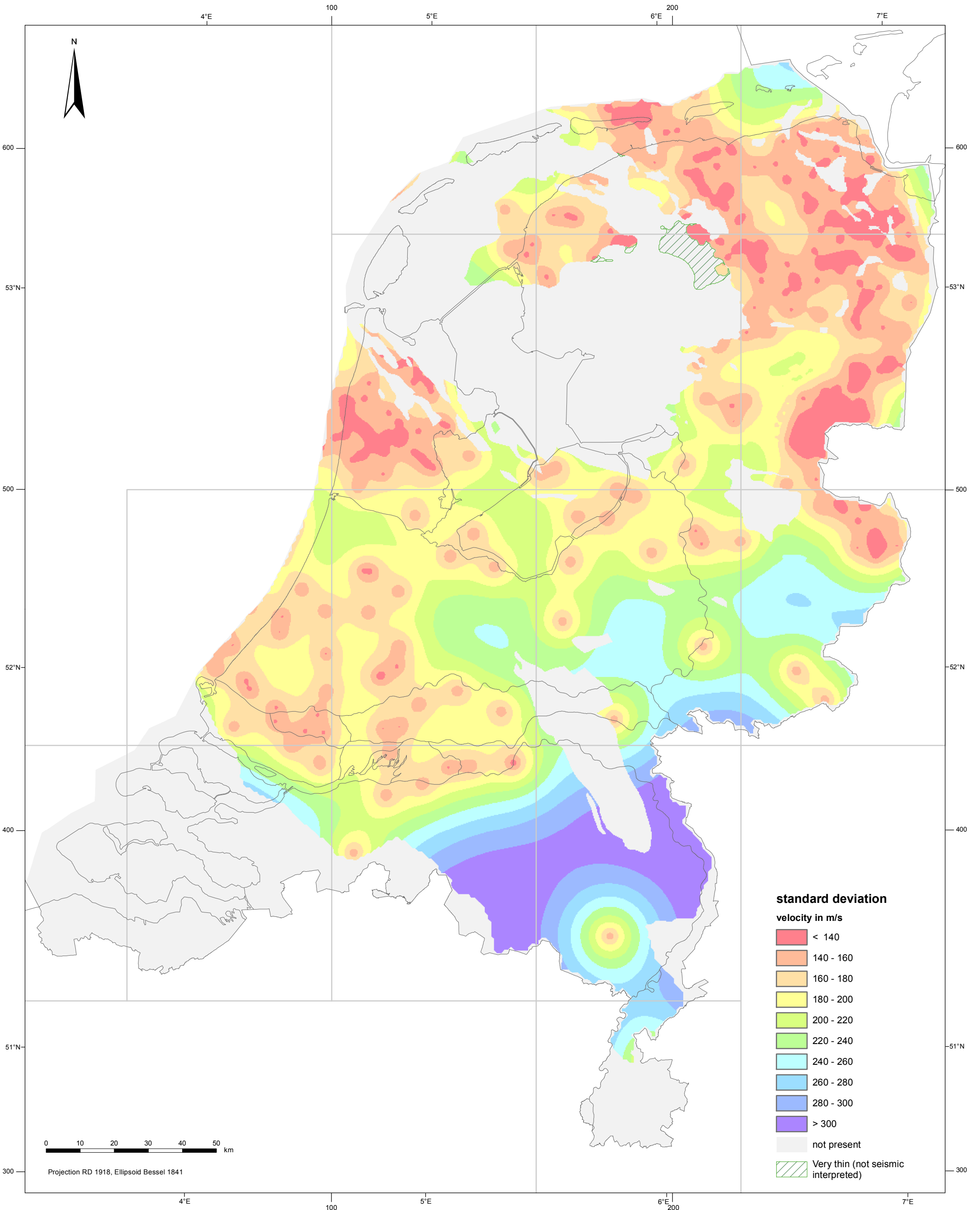
Uncertainty (standard deviation) of the velocity ( V_0 ) of the Lower Germanic Trias Group (RB)
