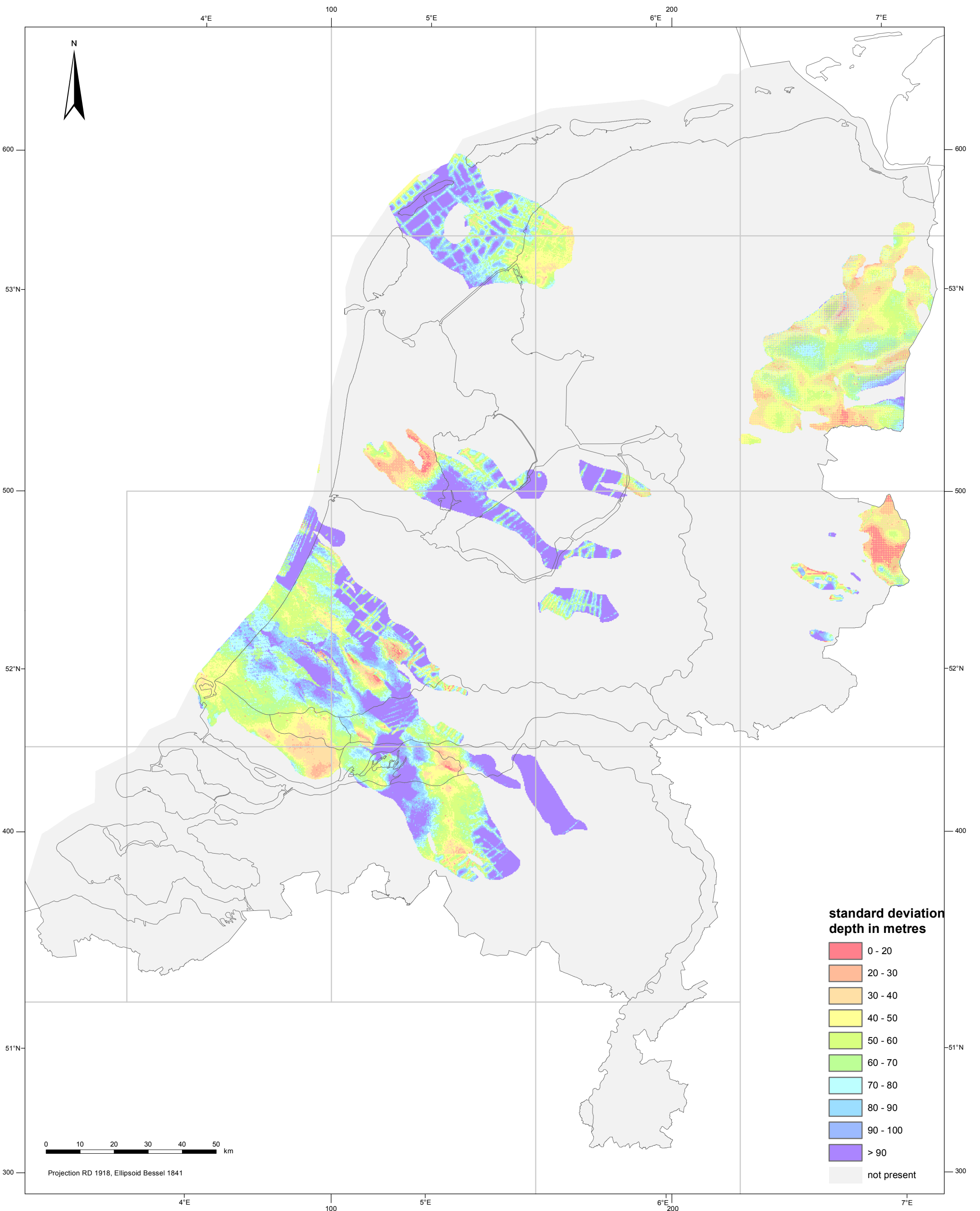
Uncertainty (standard deviation) of the depth of the base of the Schieland and Niedersachsen Groups (S)
